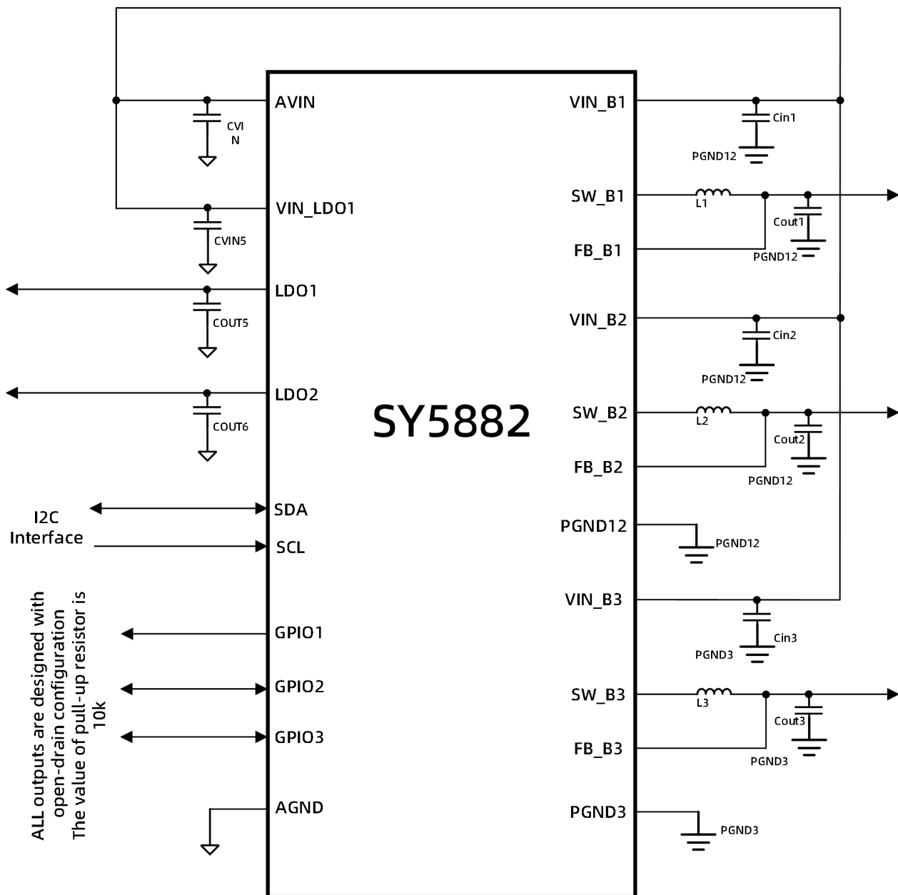
Figure 4- 1. Typical Application Circuit
